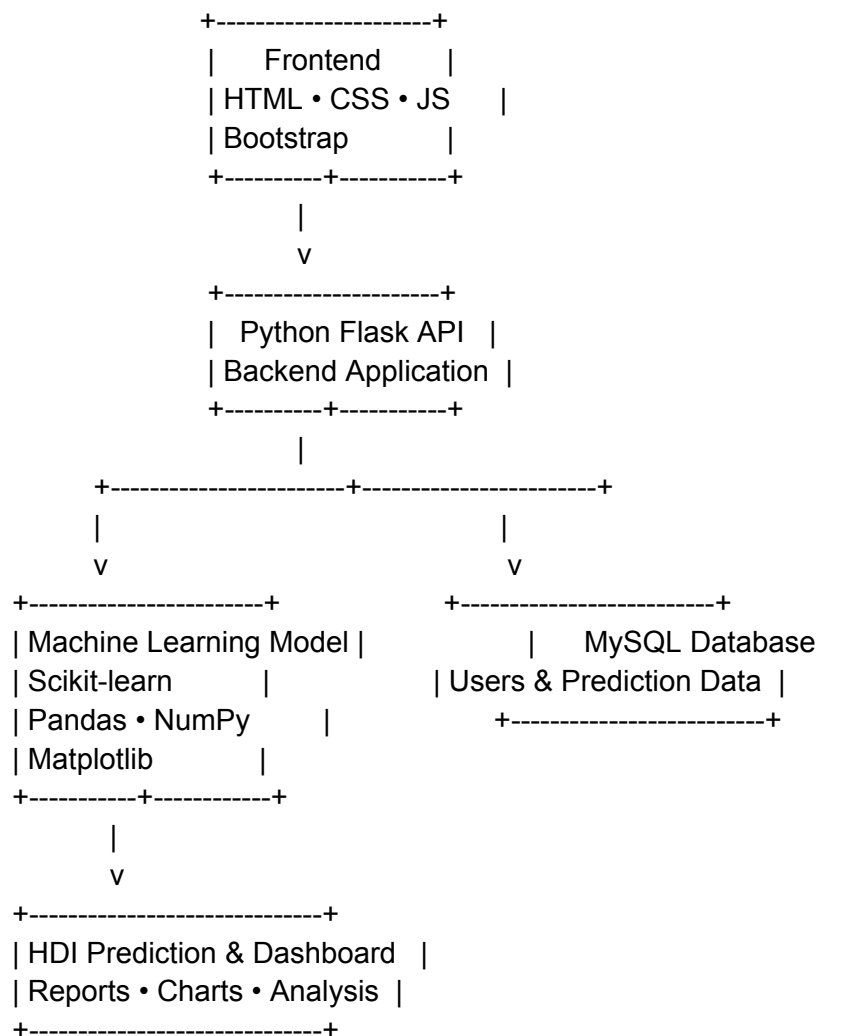
Figure 5.1: Technology Stack of the Human Development Index (HDI) Prediction System
